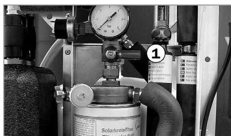
Ball valve over the solar filter closed
