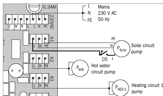
Excerpt from the wiring plan: connection of the pressure switch (DS) to the solar pump
