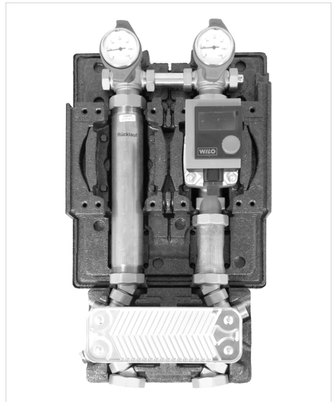
Fig. 39: Attached HK-WÜT
