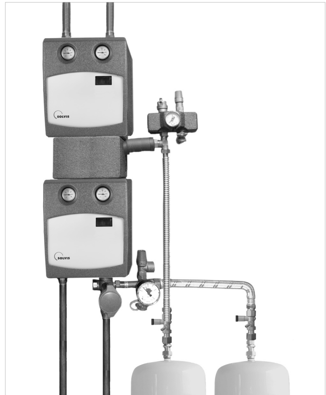
Fig. 44: Completely installed heating circuit group
