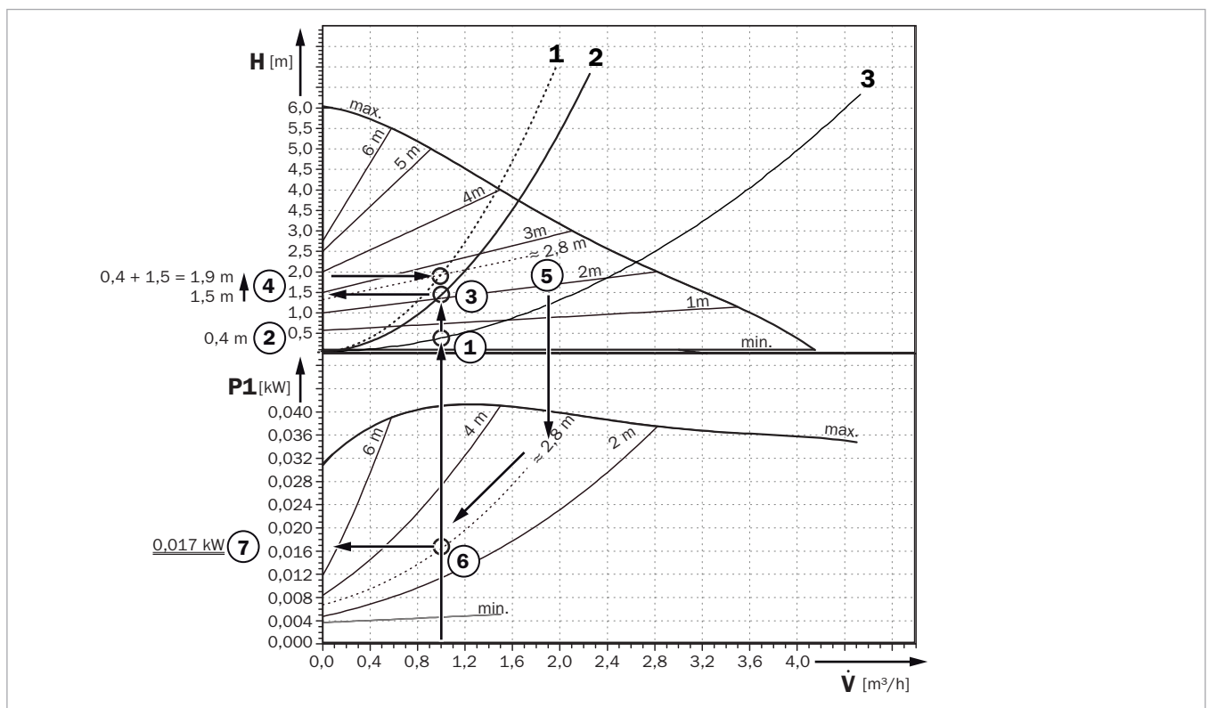
Fig. 51: Determination of the set pumping height of the secondary heating circuit with an example of a system characteristic curve
