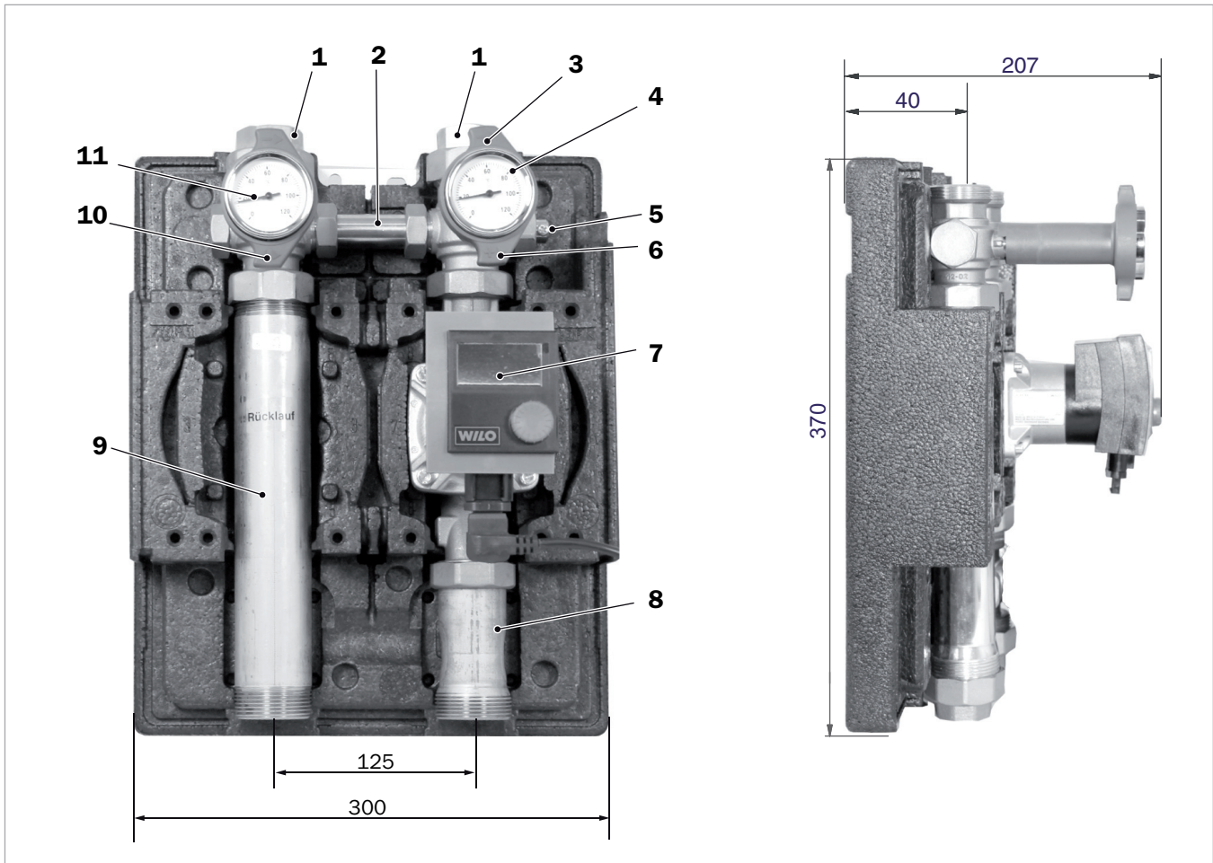
Fig. 30: HKS-FB heating circuit station
