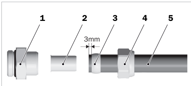
Afb.4: Montage knelkoppeling
