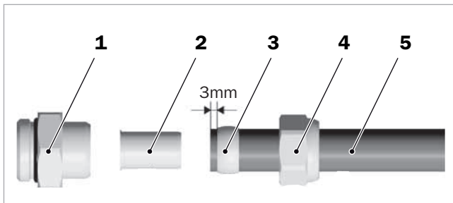
Afb.4: Montage knelkoppeling
