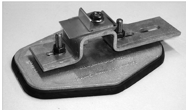
Fig. 8: Roof-mounted frame completely installed
