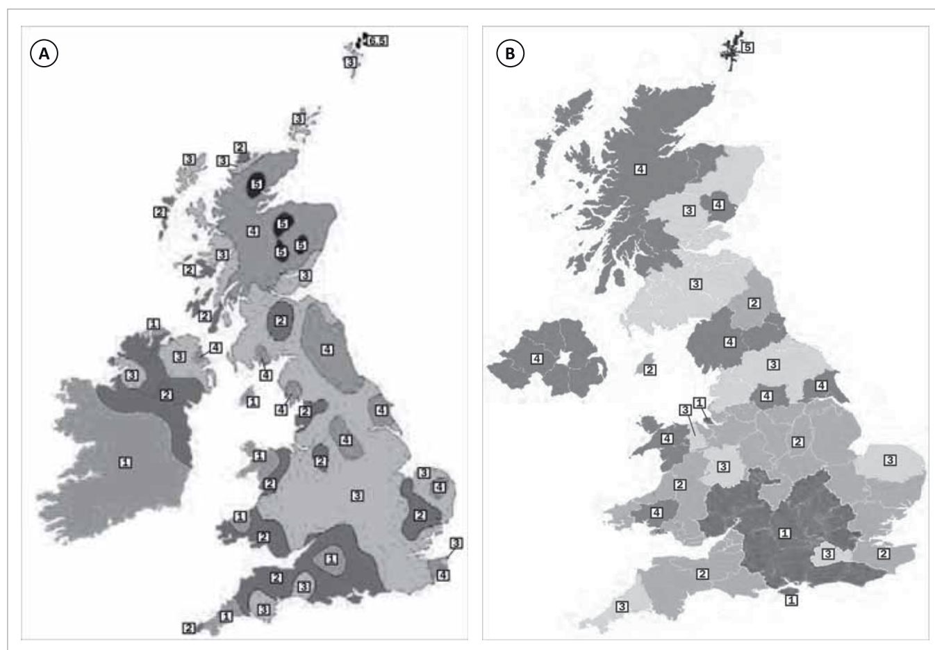
Fig. 99: Distribution of snow and wind load zones in Great Britain
