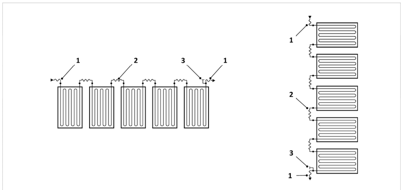
Fig. 10: SolvisCala 254 AR, horizontal and vertical series connection
