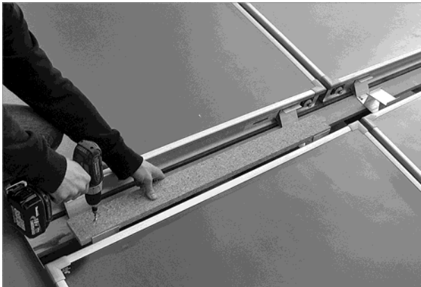
Fig. 67: Screwing intermediate flashing supports onto collector spacers
