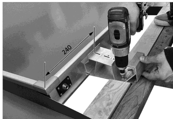
Fig. 60: Screwing on collector spacers at a distance to the left and right of the outer edge of the collector
