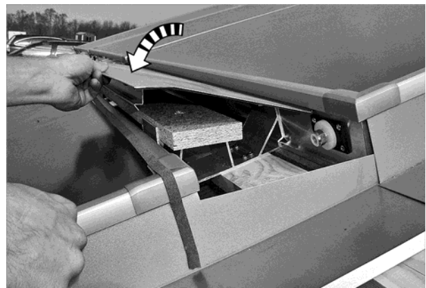
Fig. 69: Turning the first piece of intermediate flashing into the slot, positioning it and pressing it in
