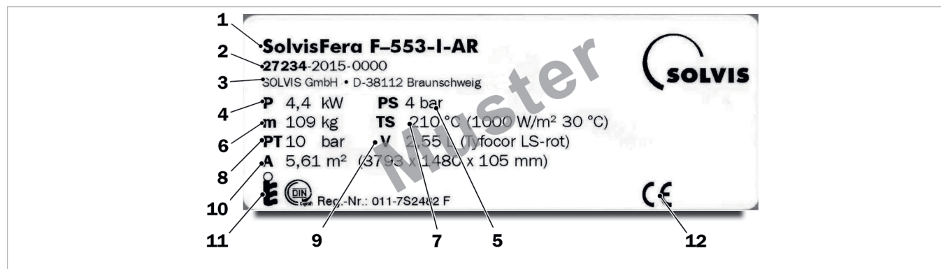
Abb. 77: Typenschildmuster SolvisFera
