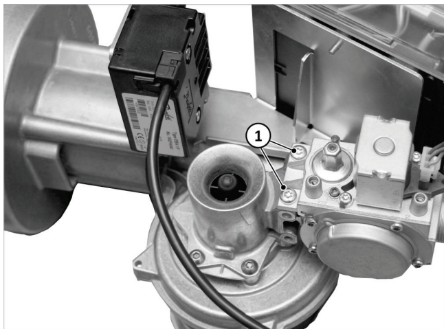
Afb. 41: Gascombiklepe demonteren
