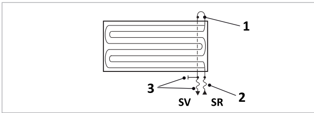
Fig. 42: SolvisFera Integral, connection cables at the bottom
