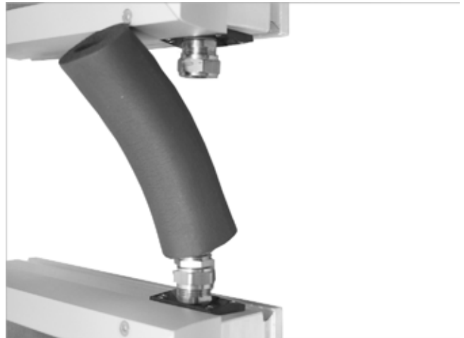
Fig. 59: VB-F-S-D-UE screwed onto the lower connection
