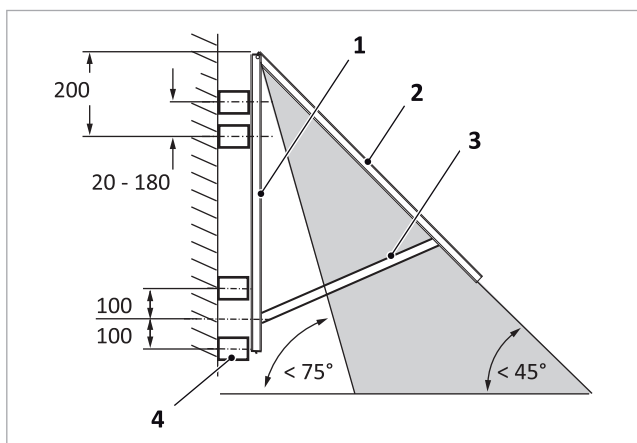
Fig. 10: Assembly of the holders on the wall
