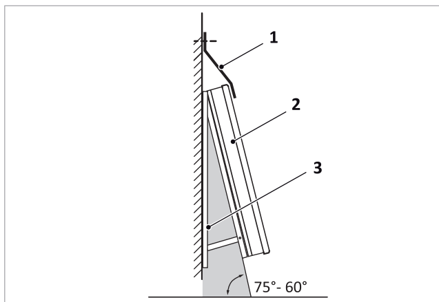
Fig. 11: Collector with cover plate
