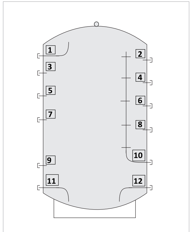
Abb. 5: Connections for the SolvisStrato 3 stratified buffer tank
