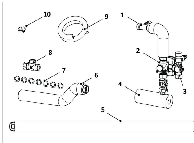
Abb. 2: Montagepack LM WP 3-W Ventil
