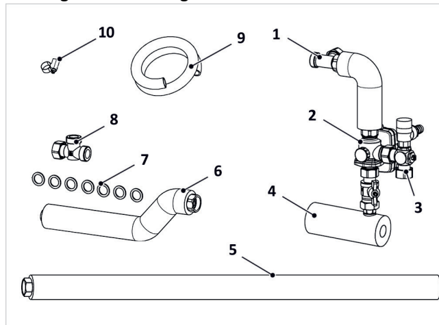
Afb. 2: montagepakket LM WP 3-W klep
