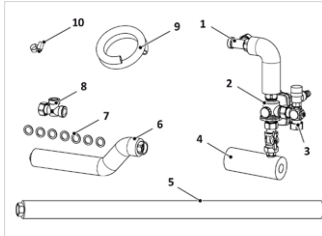
Afb. 2: montagepakket LM WP 3-W klep
