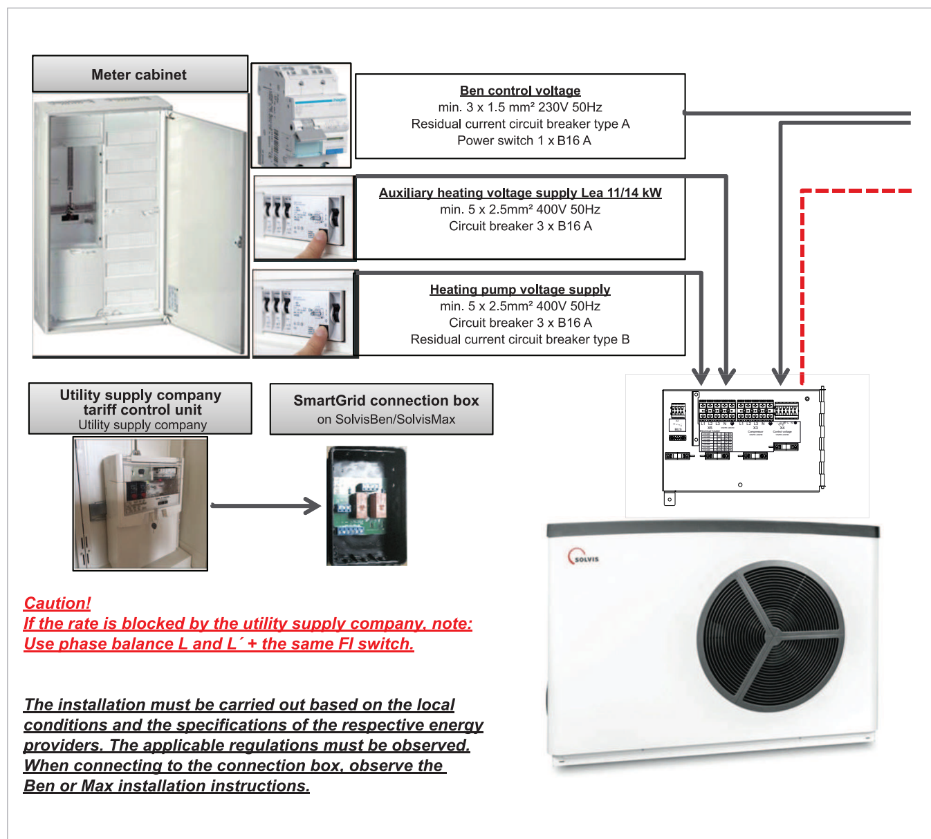
Fig. 1: Installation aid for SolvisBen HP with SolvisLea 11/14 kW and utility supply company connection – Part 1
