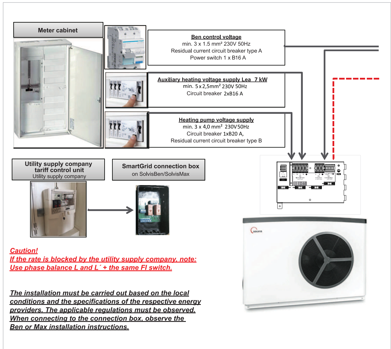
Fig. 3: Installation aid for SolvisBen HP with SolvisLea 7 kW and utility supply company connection – Part 1
