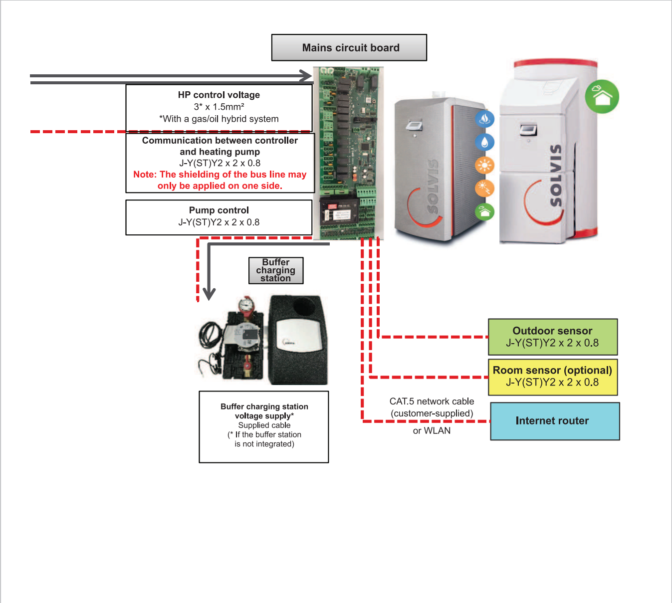
Fig. 4: Installation aid for SolvisBen HP with SolvisLea 7 kW and utility supply company connection – Part 2
