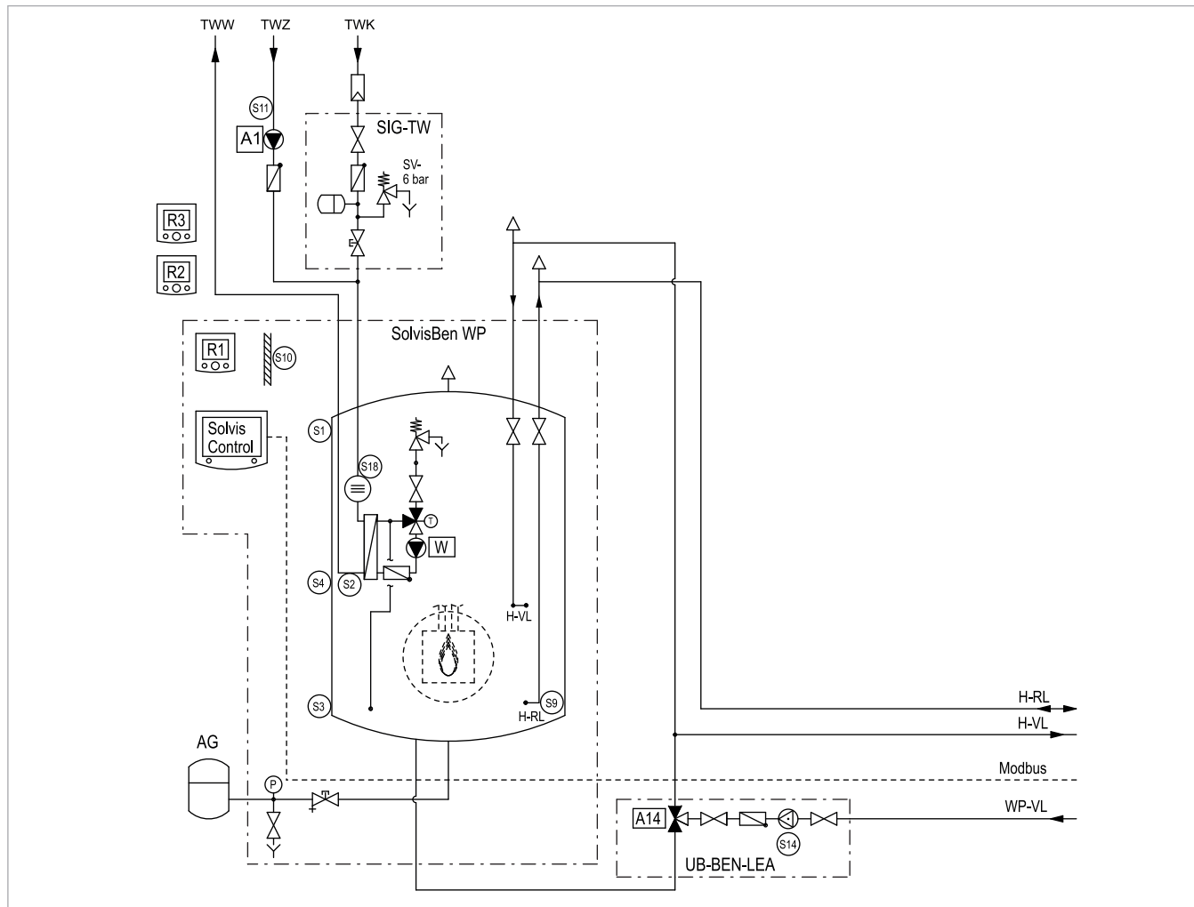
Fig. 19: SolvisBen WP with three mixed heating circuits and SolvisLea heating pump – part 1
