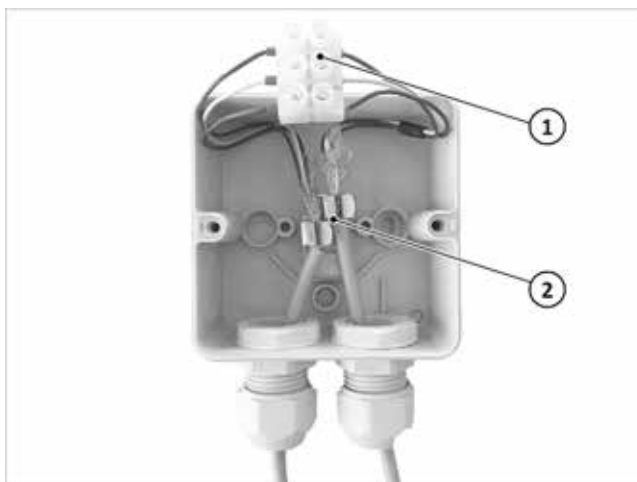
Fig. 12: Attaching the Modbus junction box
