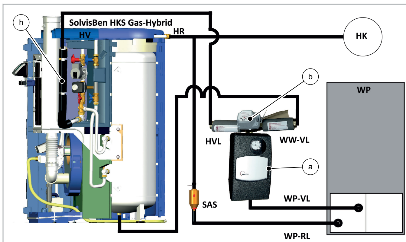
Fig. 9: Panoramica collegamento SolvisLea a SolvisBen HKS Gas-Hybrid
