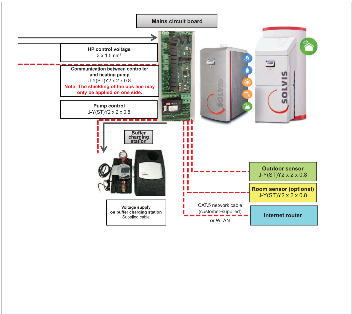
Fig. 2: Installation aid for SolvisBen / SolvisMax Hybrid with SolvisLea Eco 8 kW and utility supply company connection – Part 2
