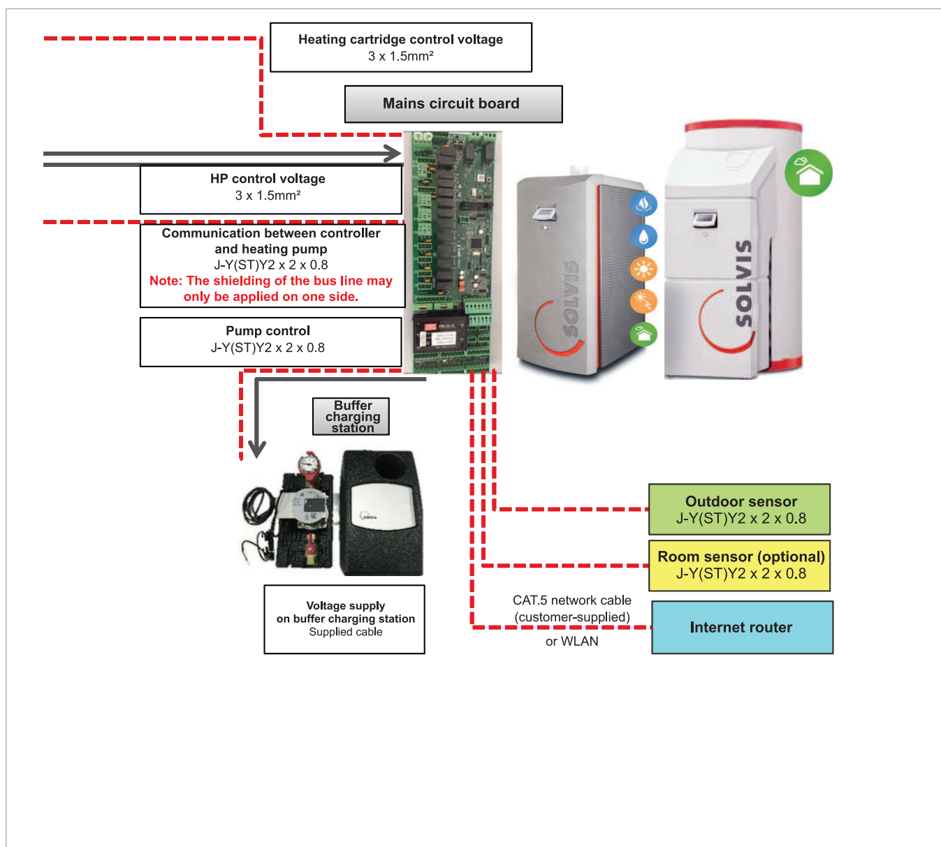
Fig. 4: Installation aid for SolvisBen / SolvisMax HP heating cartridge with SolvisLea Eco 8 kW and utility supply company connection – Part 2
