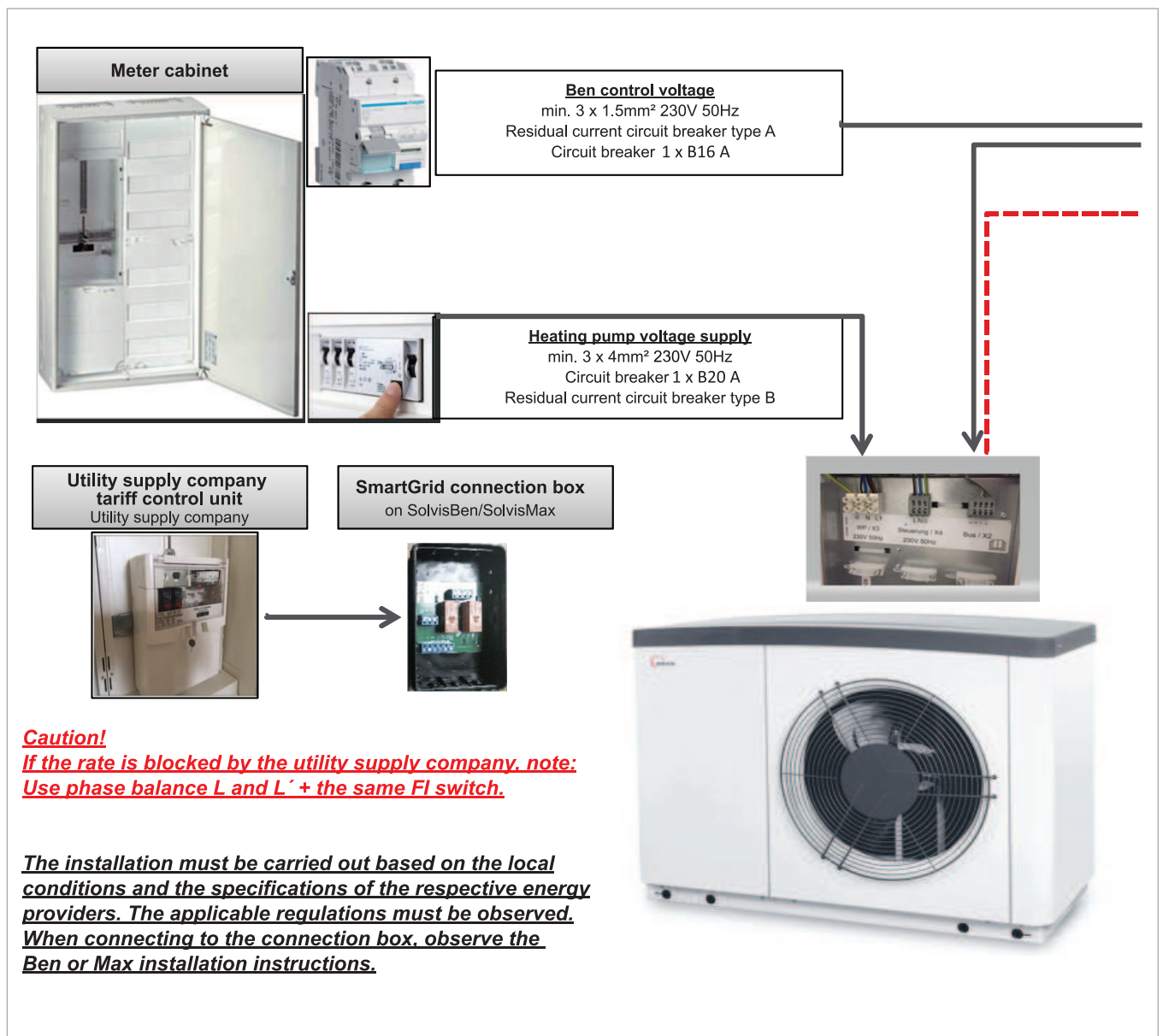
Fig. 1: Installation aid for SolvisBen / SolvisMax Hybrid with SolvisLea Eco 8 kW and utility supply company connection – Part 1
