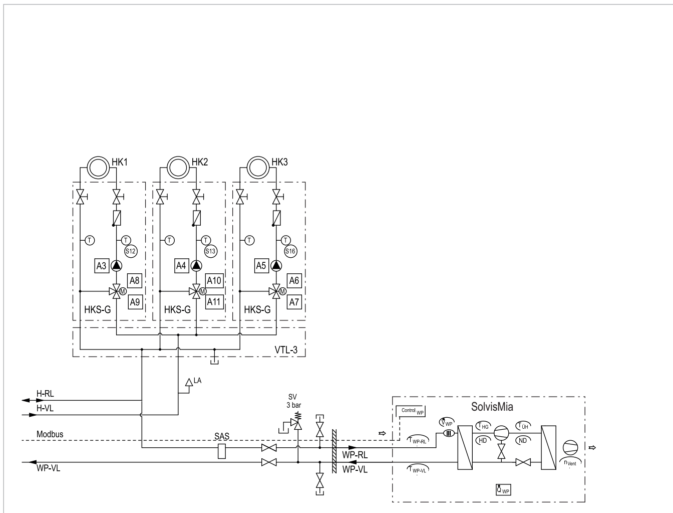
Fig. 26: SolvisBen WP with three mixed heating circuits and SolvisMia heating pump – part 2
