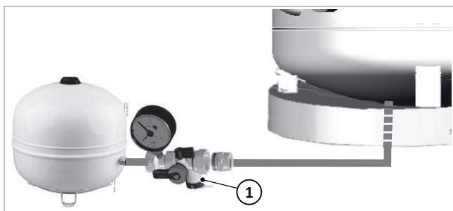
Fig. 11: Boiler filling and emptying valve on the MEV connection group
