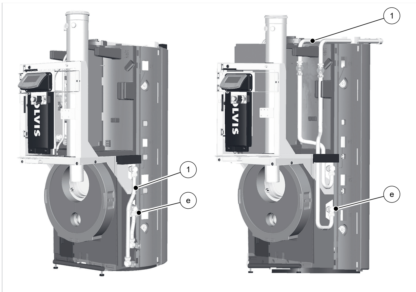
Fig. 3: Ext. connections for HCS routed down (left side) and routed back (right side)
