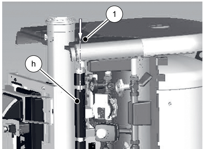
Fig. 8: Cutting the EPP cover
