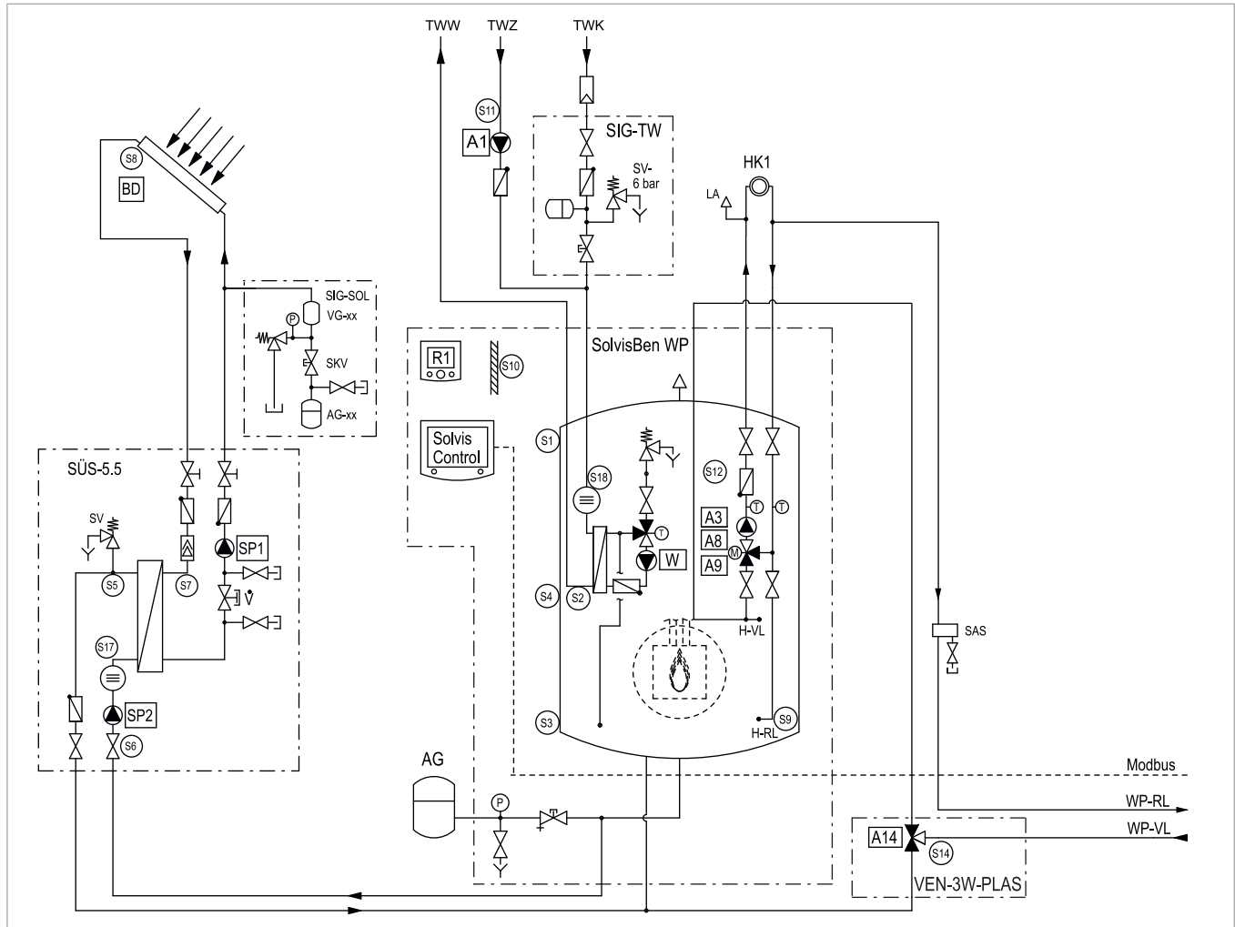
Fig. 12: SolvisBen Gas/Oil Hybrid with integrated heating circuit station, solar system and Solvis heating pump – part 1
