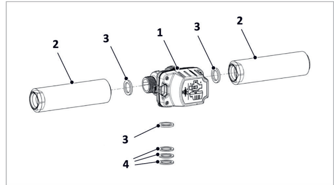
Fig. 2: Switching valve group with seals (pre-assembled)
