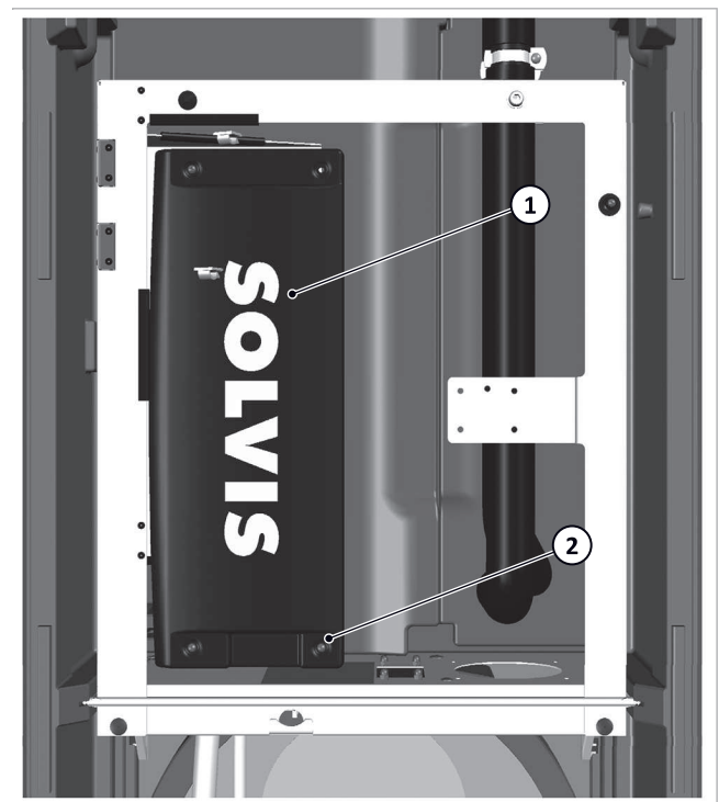
Fig. 10: Attach the cover of the mains circuit board
