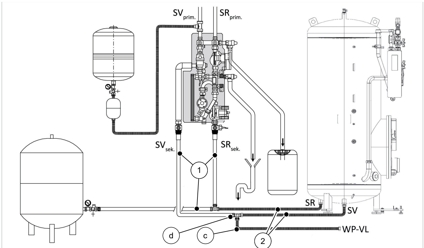
Fig. 6: Position of the 3-way switching valve (connections on the right)
