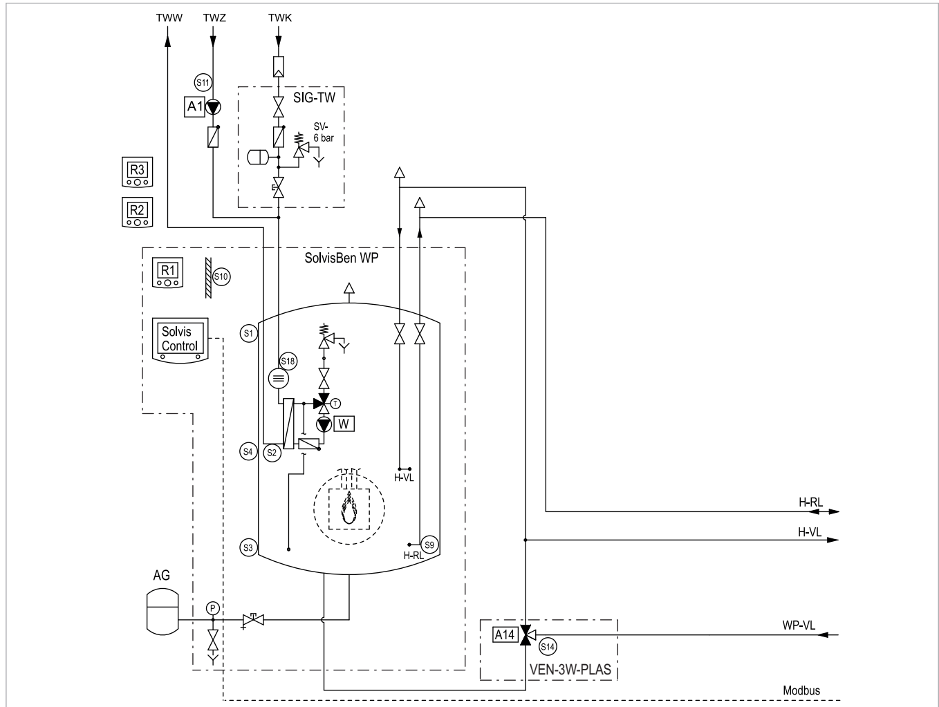
Fig. 14: SolvisBen Gas/Oil Hybrid with three mixed heating circuits and Solvis heating pump – part 1
