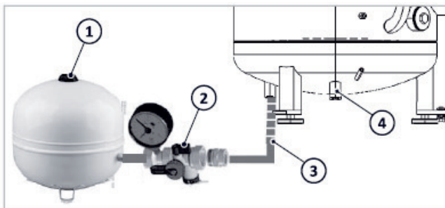
Fig. 7: Connecting the HW flow to the storage tank (without solar system)
