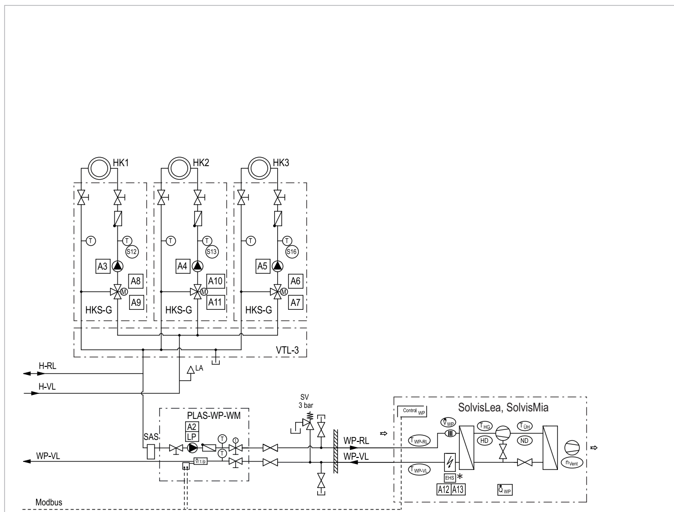
Fig. 15: SolvisBen Gas/Oil Hybrid with three mixed heating circuits and Solvis heating pump – part 2
