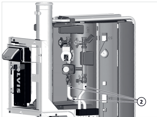
Fig. 4: Removing the pipe sections (2)
