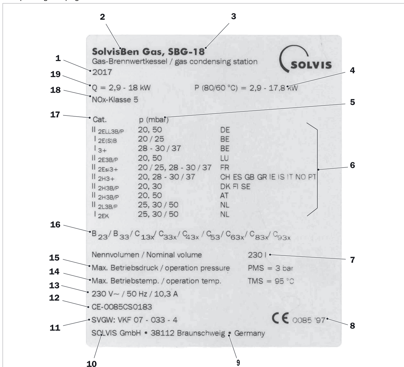
Fig. 159: Modello targhetta SolvisBen Gas
