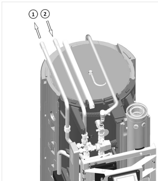
Fig. 31: Attacco posteriore TWK/TWW
