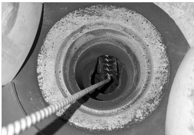
Abb. 27: Brennkammer/Rost reinigen
